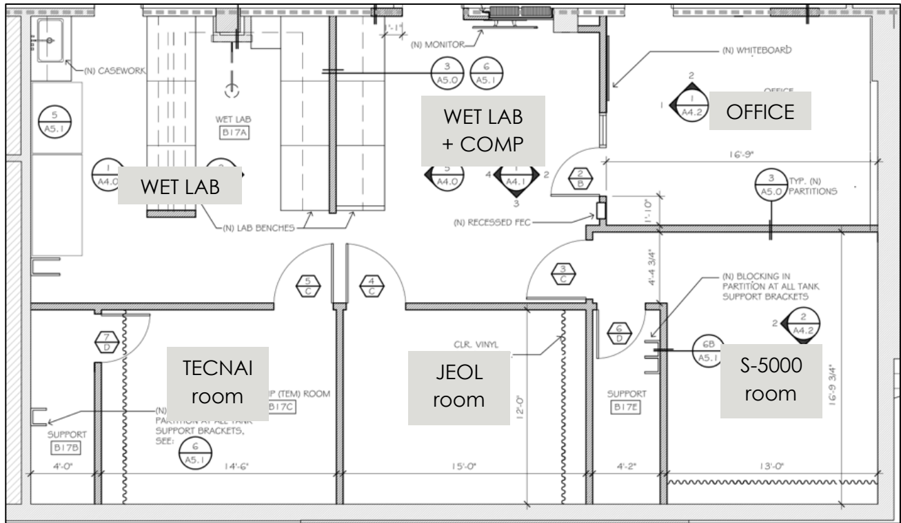
Above: Barker Hall Room 17 layout. Main EML suite w/ office, wet lab, & 3 microscope rooms
